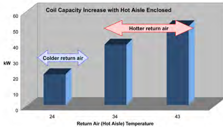
Fig. 3 Effect of warmed return air temperature on coil capacity
