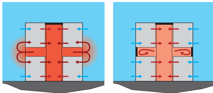
Fig. 1 Blanking panels (right diagram) prevent the recirculation of hot exhaust air (left diagram).
