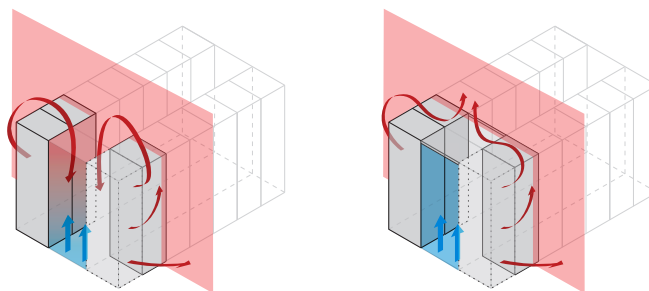
Fig. 2 Sealing the aisle to prevent hot air recirculating.
