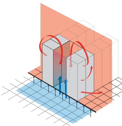
Fig.2 Conventional air supply from raised floor is inadequate to stop recirculation of hot aisle air.
