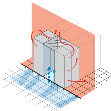
Fig.3 Cold aisle enclosure stops recirculation but relies on sufficient air supply from the raised floor. Obstructions in the floor void prevent sufficient delivery of cooled air.
