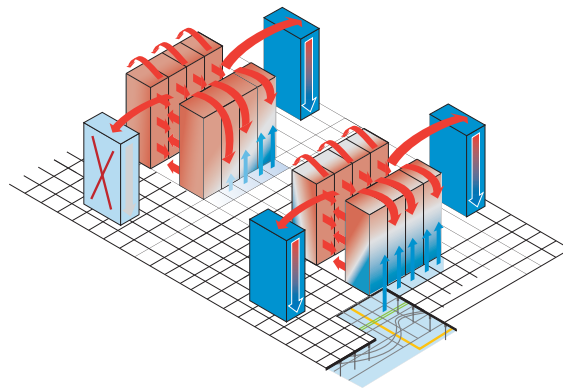
Fig.1 Even in well laid out rooms with a CRAC at the end of each hot aisle, a single unit failure results in unpredictable hot spots in front of the IT servers.
