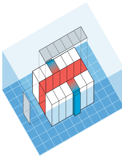
Fig.6 Hot aisle enclosure maximizes coil capacity, assures redundancy and can reduce chiller power.
