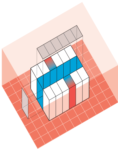
Fig.5 Enclosed cold aisle eliminates uncertainty of raised floor air distribution.
